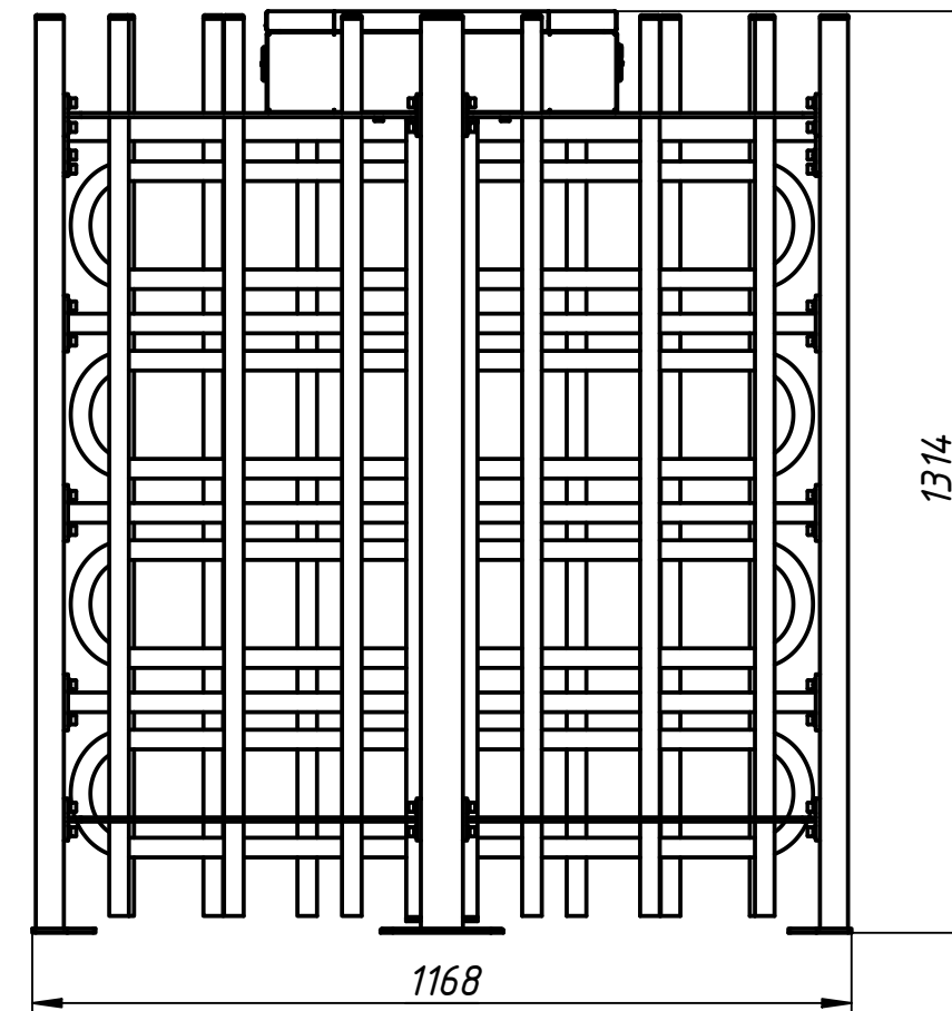
Installation tamplate
