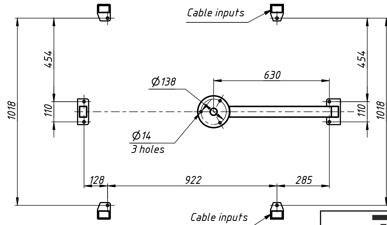
Installation tamplate
